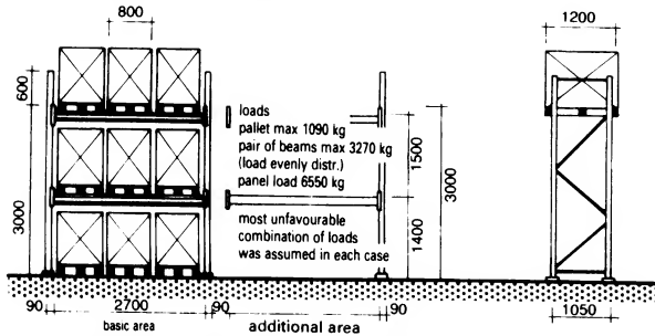
2 Pallet racking system for Euro pallets
